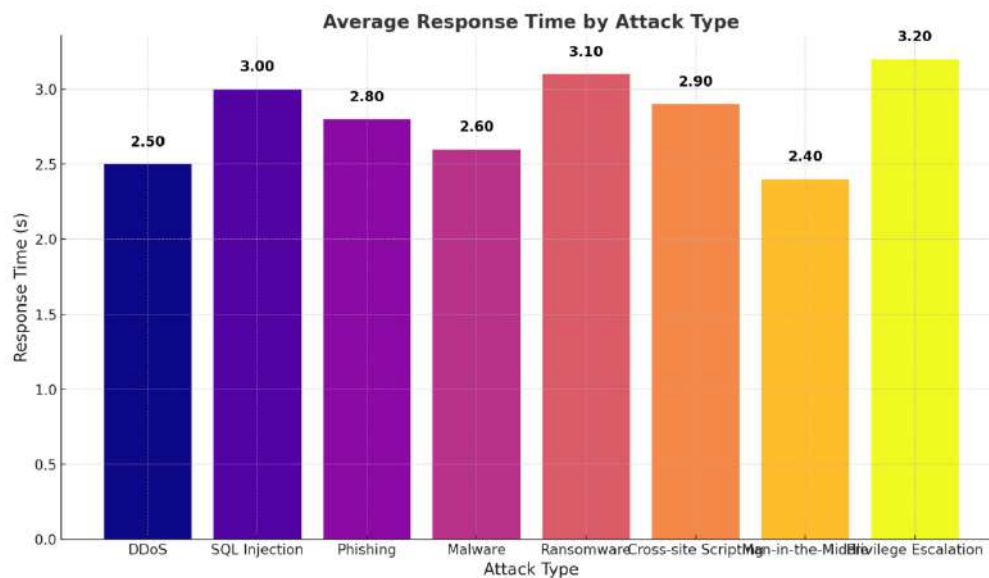
Figure 3 Average Response Time by Attack Type
